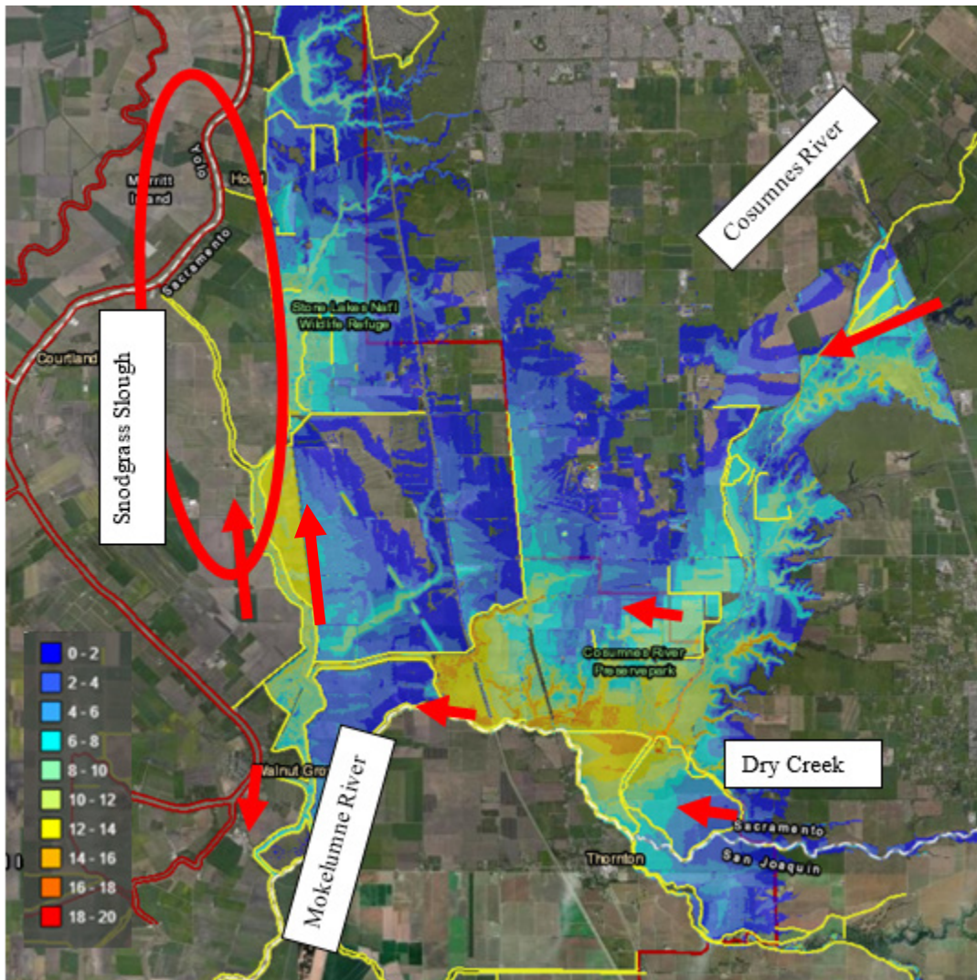
Figure 4-4: 1997 Storm Event Flood Depths Experienced and Modeled by Sacramento County North Delta Hydraulic Model
