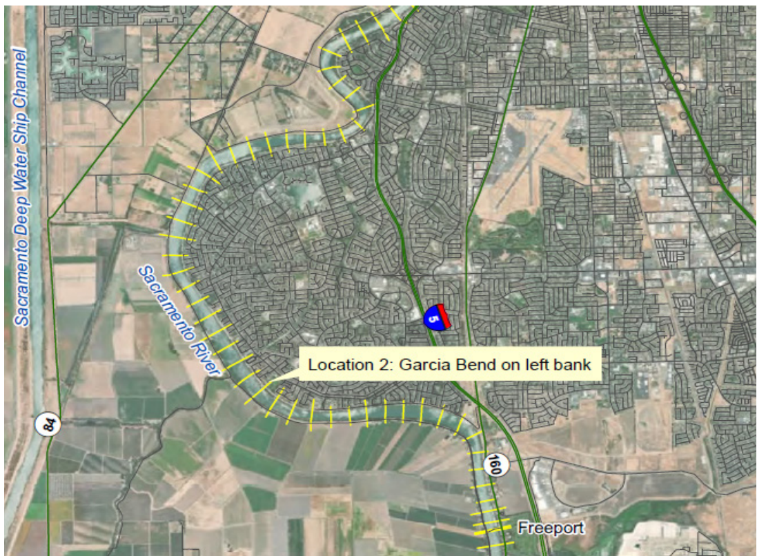
Figure 4-7: High-Water Mark Location 2 – Left Bank at Garcia Bend
