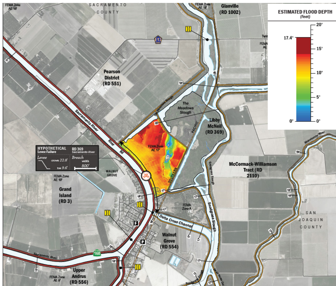
Figure 5-4: Estimated Maximum Flood Depths for RD 369, Locke from Levee Breach Occurring Along the Left Bank of the Sacramento River
