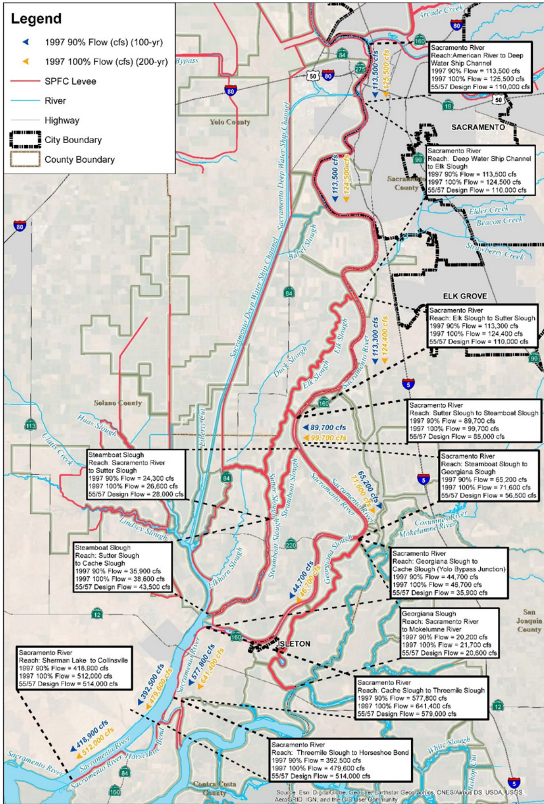
Figure 4-2: Lower Sacramento River Hydraulic Model Results for Existing Conditions Compared to the USACE 1957 Design Flows
