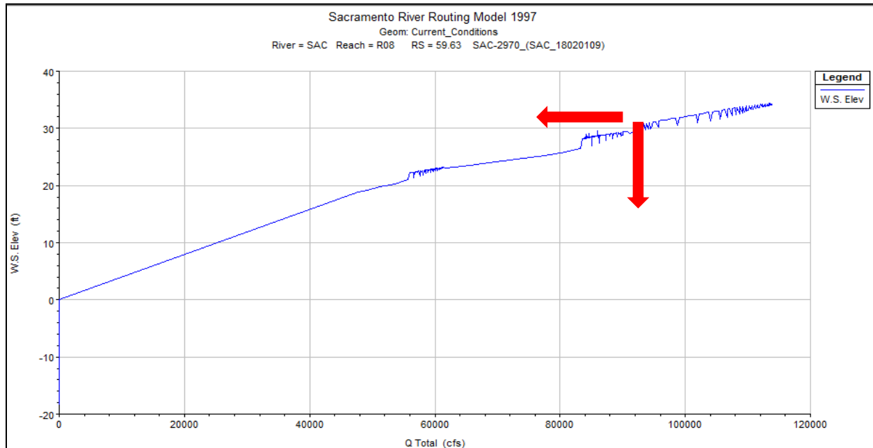
Figure 3-4: Hydraulic Model Rating Curve at I Street
