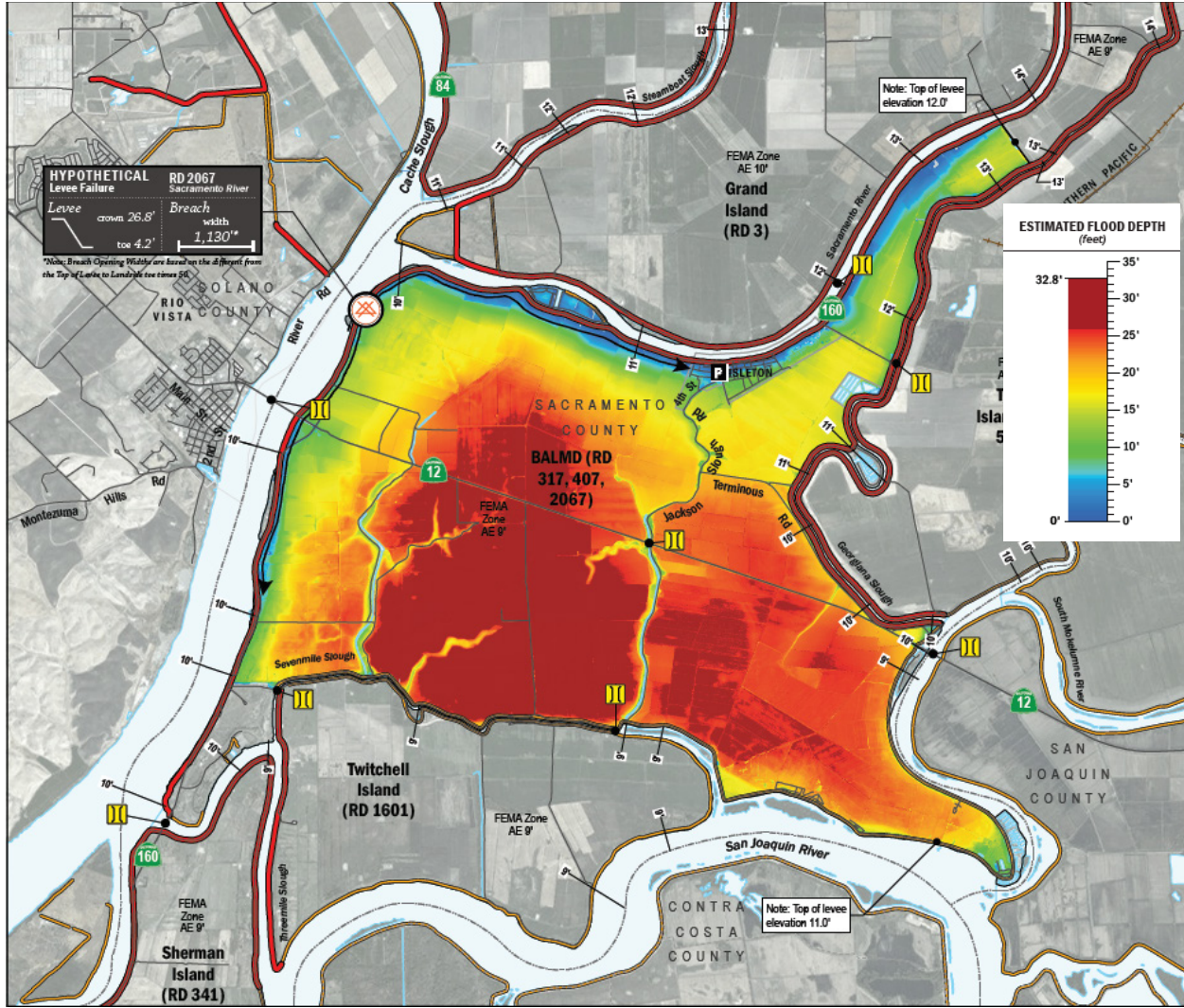
Figure 5-7: Estimated Maximum Flood Depths for BALMD, City of Isleton from Levee Breach Occurring Along the Left Bank of the Sacramento River
