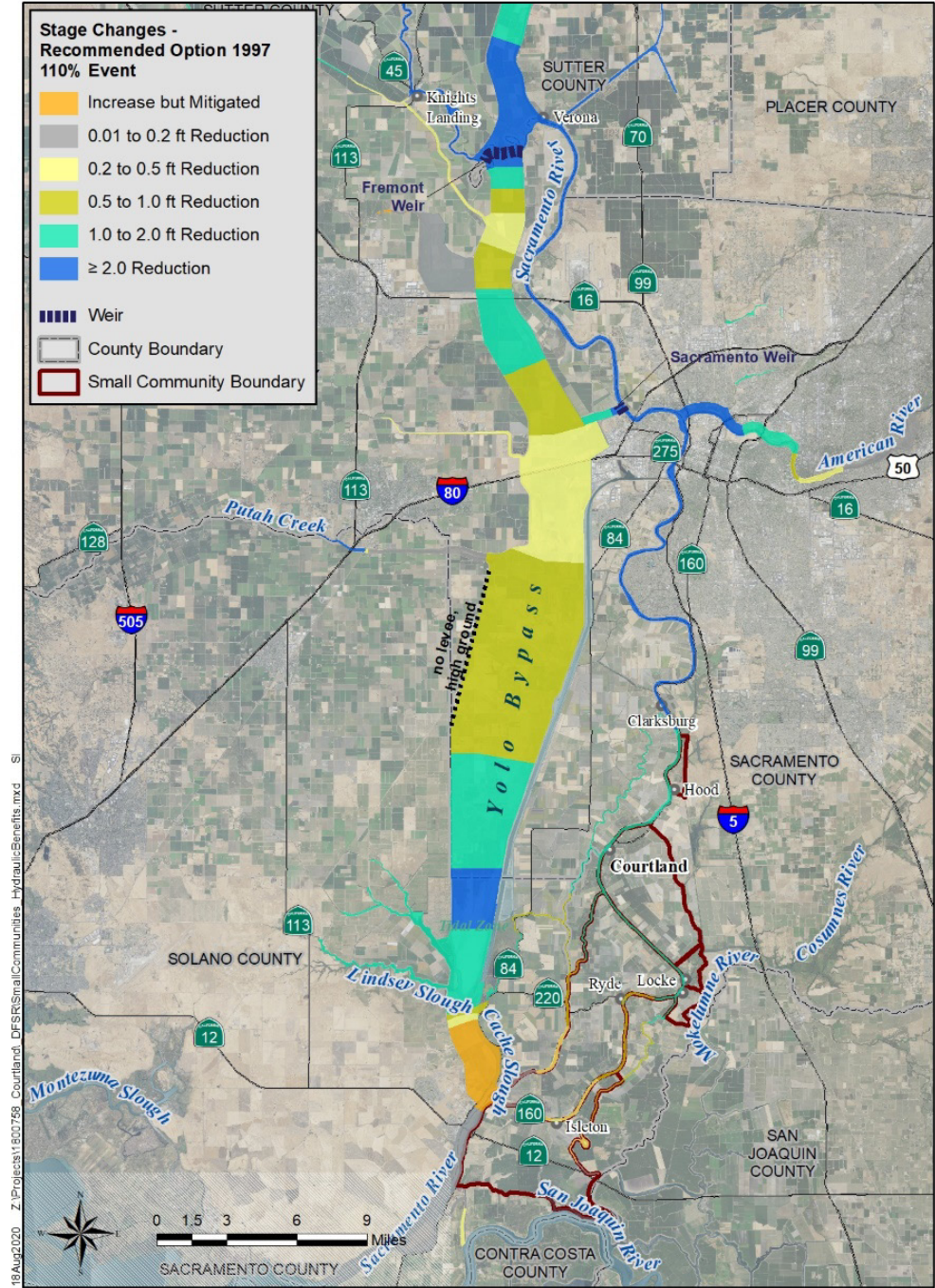
Figure 4-3: Stage Reduction Hydraulic Benefits of 2017 CVFPP System-Wide Bypass Improvements to Delta Legacy Communities in Sacramento County
