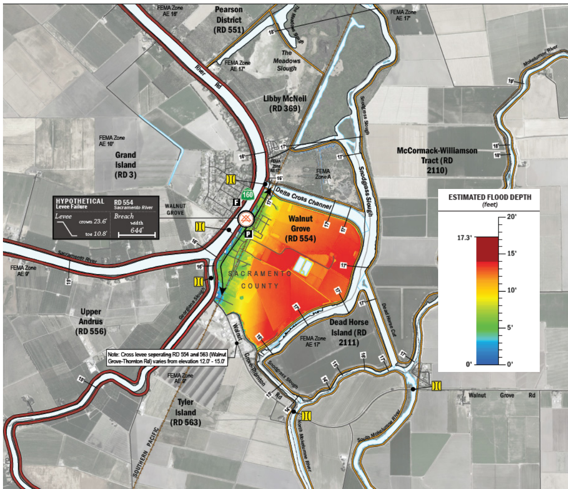
Figure 5-5: Estimated Maximum Flood Depths for RD 554, Walnut Grove (East) from Levee Breach Occurring Along the Left Bank of the Sacramento River
