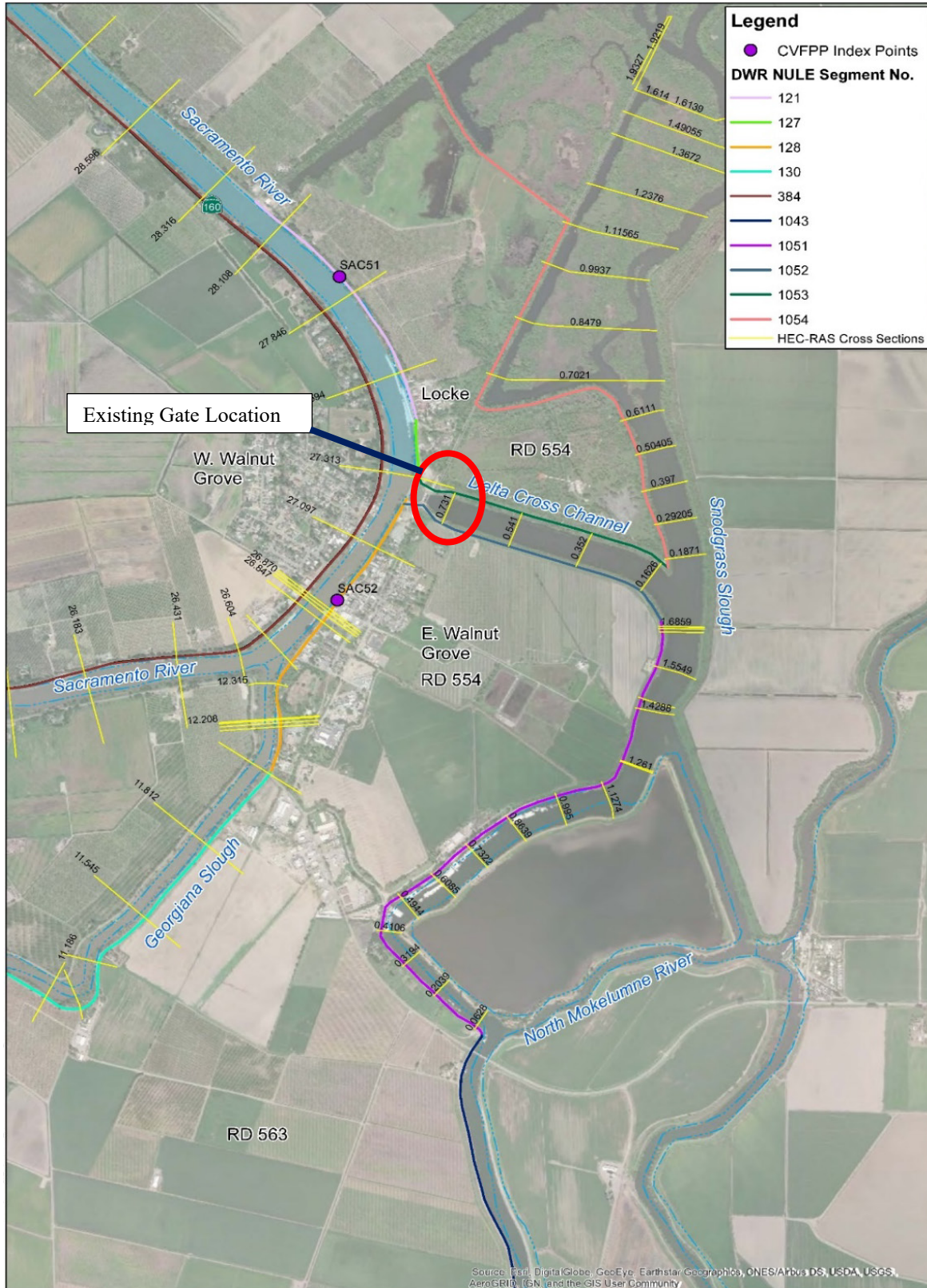
Figure 4-20: East Walnut Grove CVFED Cross-Section & NULE Reach Map at Delta Cross Channel
