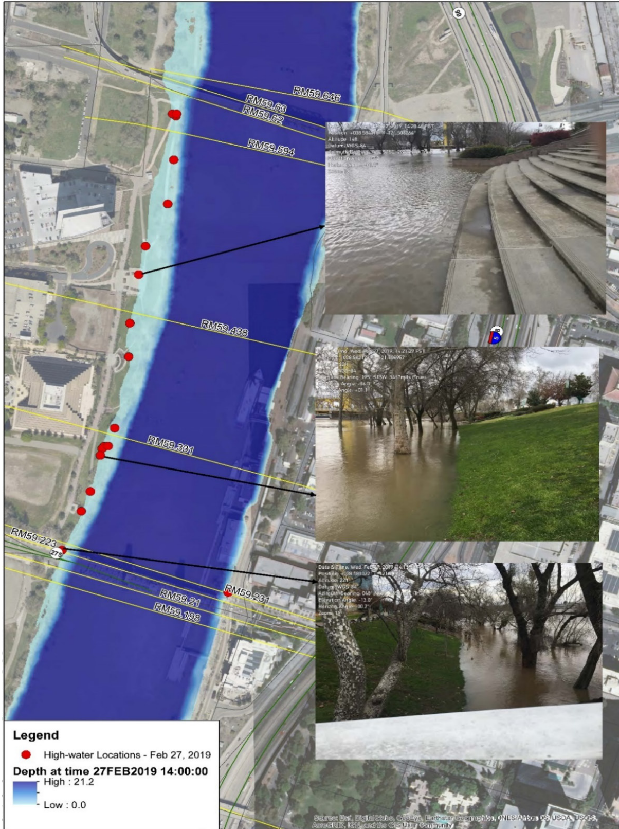
Figure 4-9: High-Water Marks at Location 1 – Sacramento, Feb 27, 2019 at 14:00
