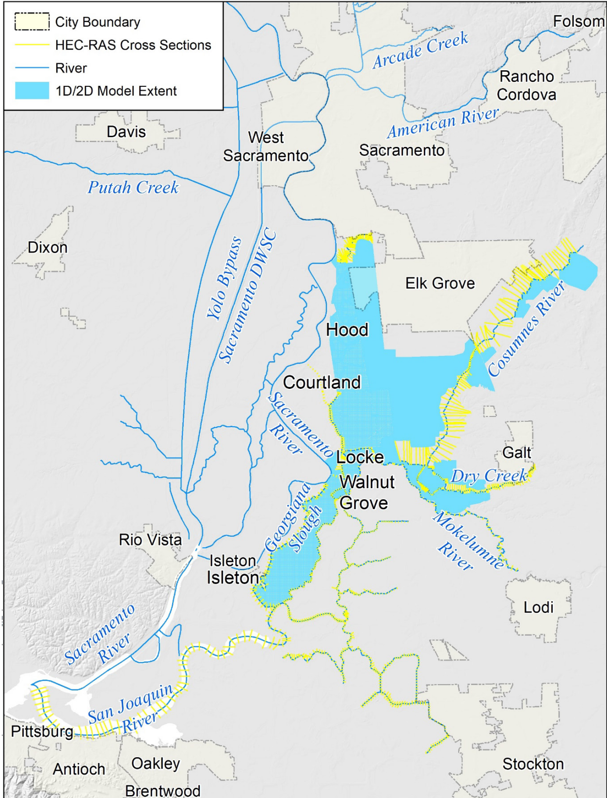
Figure 1-3: Sacramento County North Delta System Model Schematic
