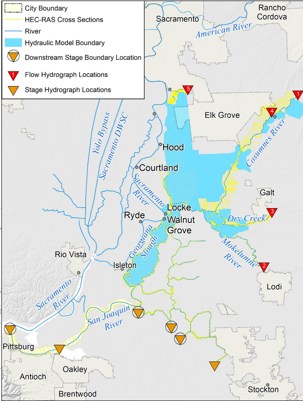
Figure 2-5: Boundary Locations of Sacramento County's North Delta System Hydraulic Model
