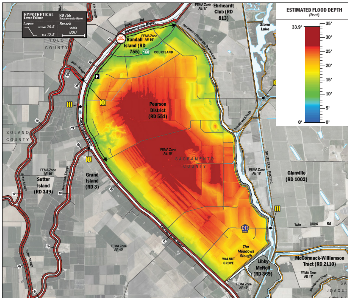
Figure 5-3: Estimated Maximum Flood Depths for RDs 551 & 755, Courtland from Levee Breach Occurring Along the Left Bank of the Sacramento River
