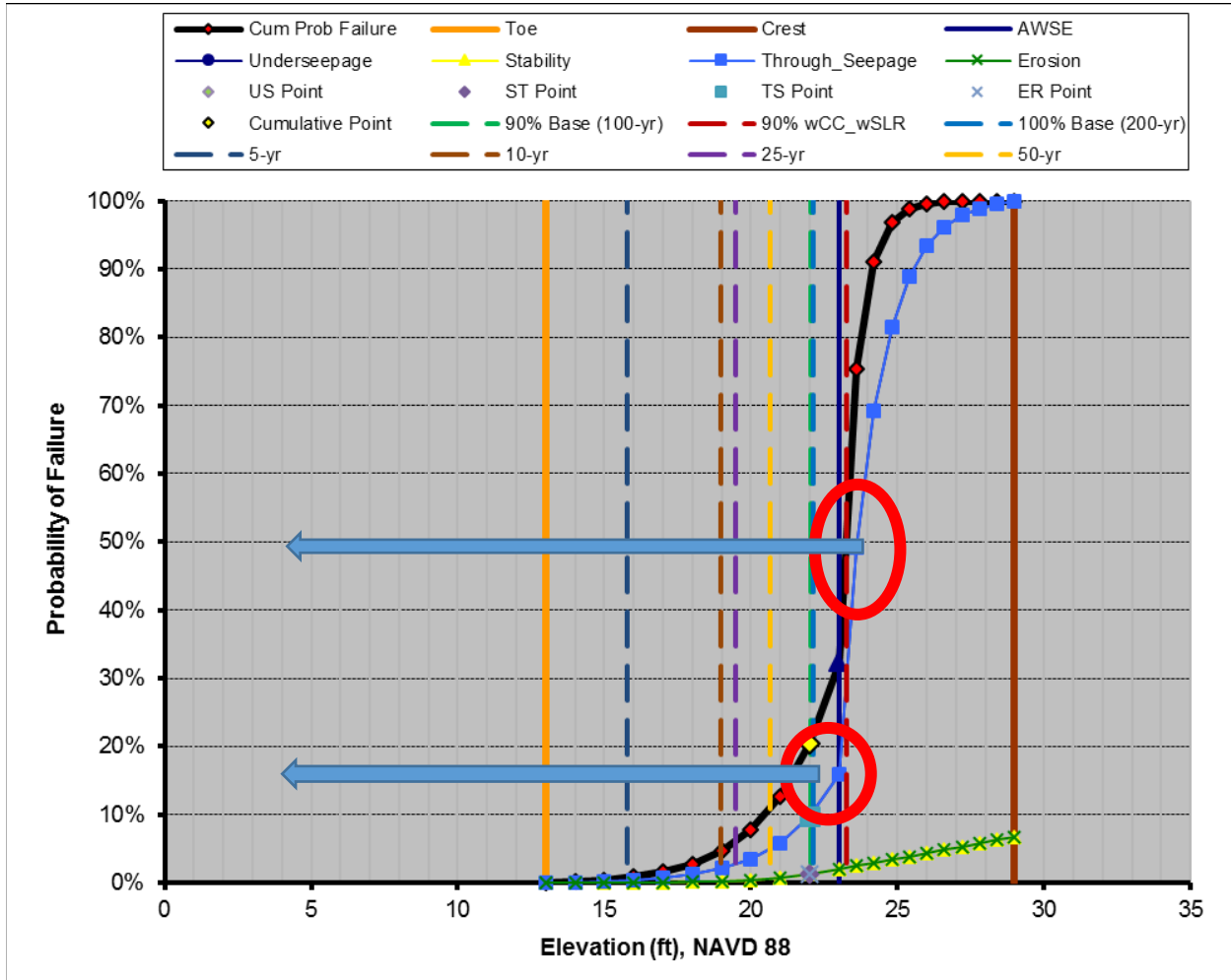
Figure 6-1: Typical Levee Performance Curve vs. Estimated Flood Stages at Hood
