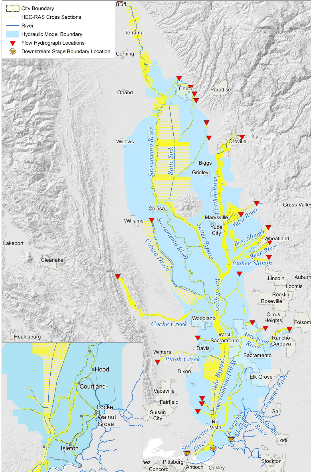
Figure 2-4: Flow and Stage Hydrograph Boundary Conditions for the DWR CVFED Sacramento River System Hydraulic Model
