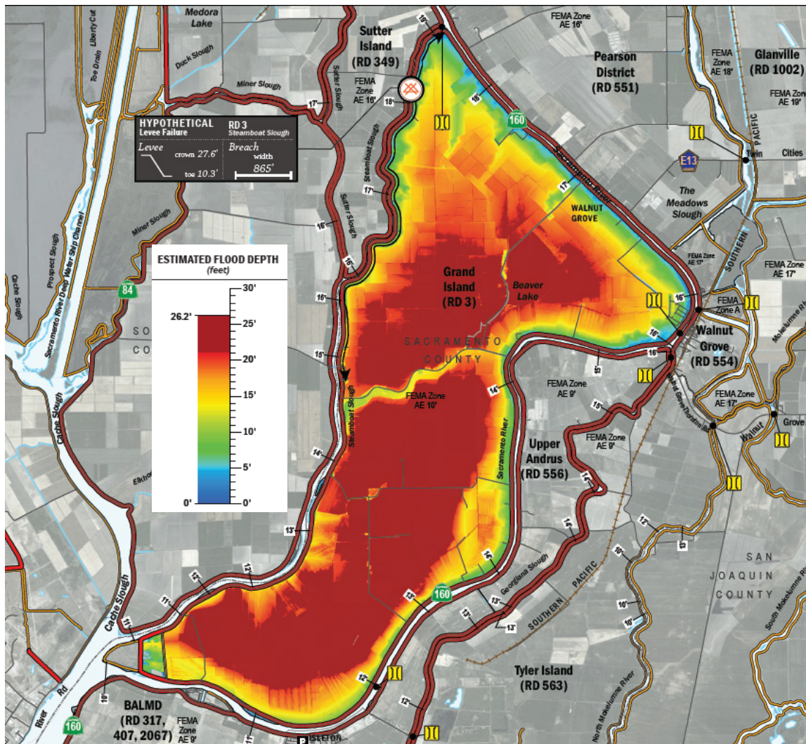
Figure 5-6: Estimated Maximum Flood Depths for RD 3, Ryde/Walnut Grove (West) from Levee Breach Occurring Along the Left Bank of Steamboat Slough
