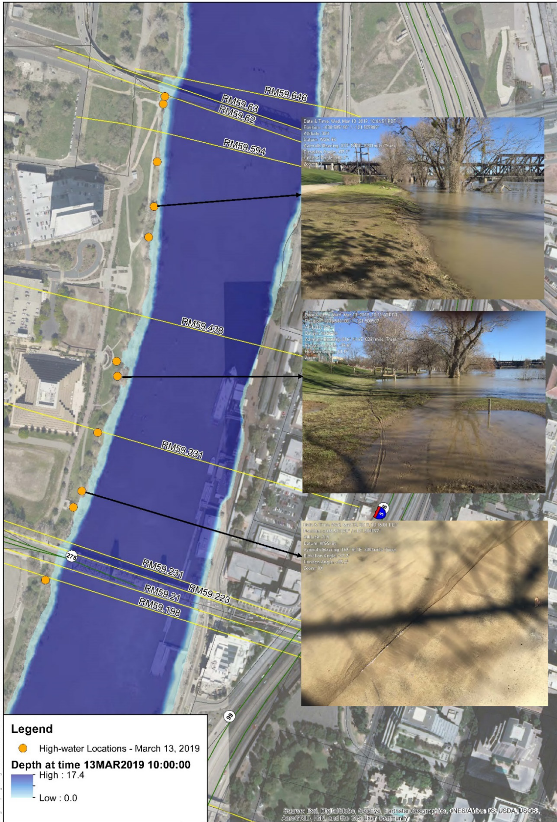
Figure 4-11: High-water Marks at Location 1 – Sacramento, Mar 13, 2019 at 10:00
