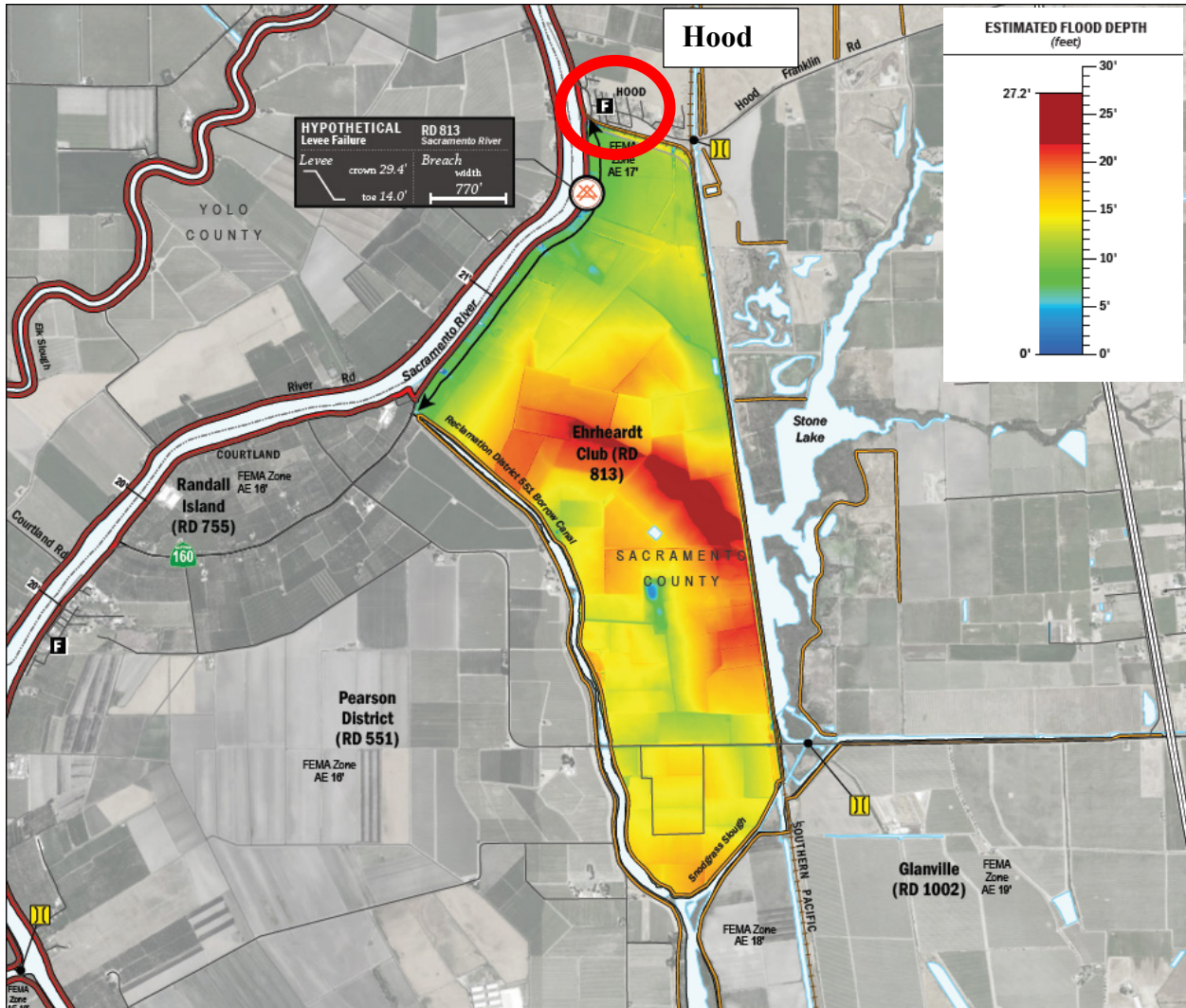
Figure 5-2: Estimated Maximum Flood Depths for RD 813 South of Hood from Levee Breach Occurring Along the Left Bank of the Sacramento River
