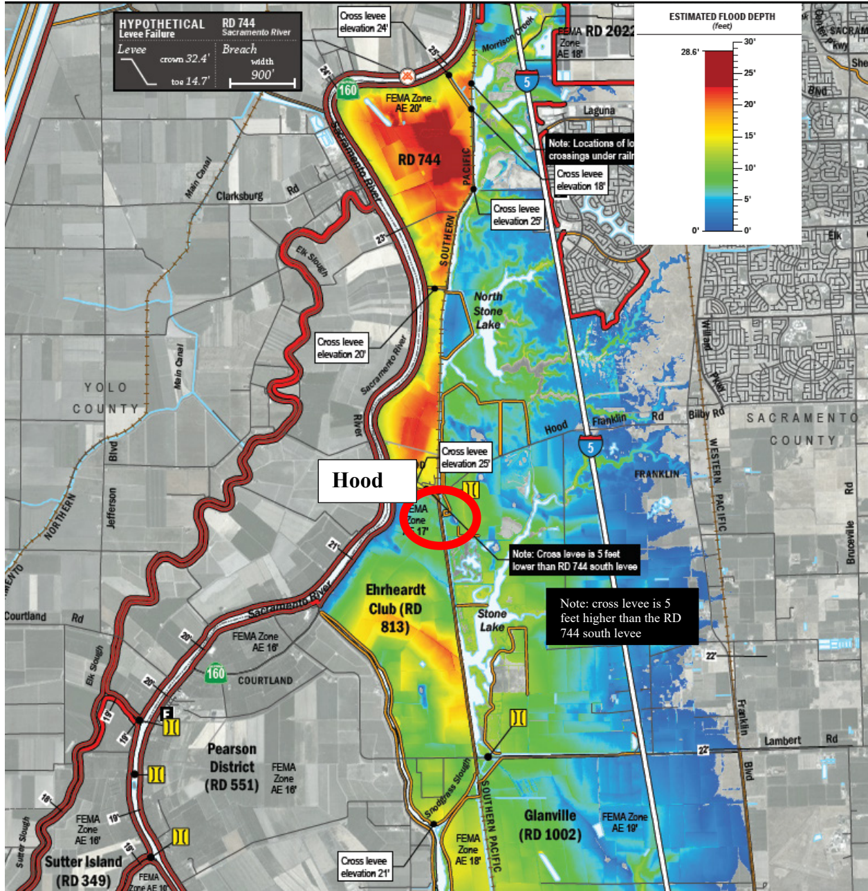
Figure 5-1: Maximum Flood Depths in Hood and Surrounding Areas from Levee Breach Occurring Upstream in RD 744 Along the Left Bank of the Sacramento River, North of Hood
