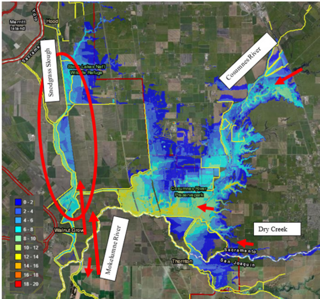
Figure 4-5: 2017 Storm Event Flood Depths Experienced and Modeled by Sacramento County North Delta Hydraulic Model
