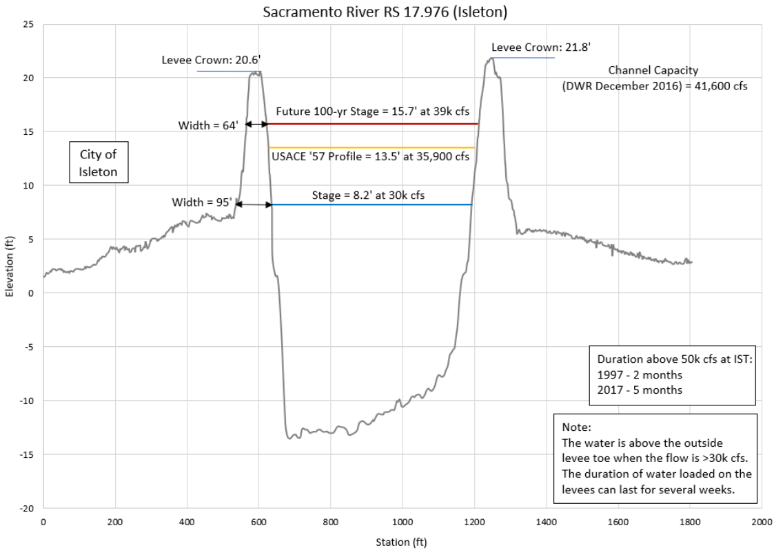
Figure 4-19: Cross Section Sta. 17.976 at Isleton Viewing Downstream
