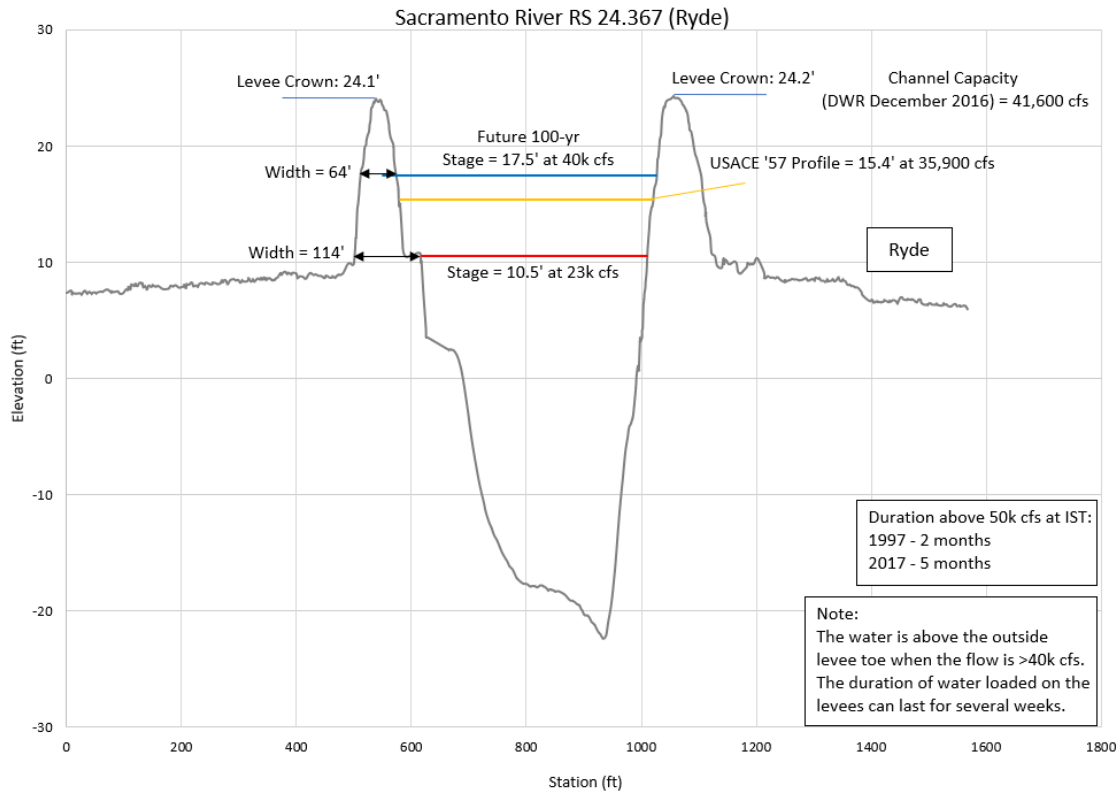
Figure 4-18: Cross Section Sta. 24.367 at Ryde Viewing Downstream
