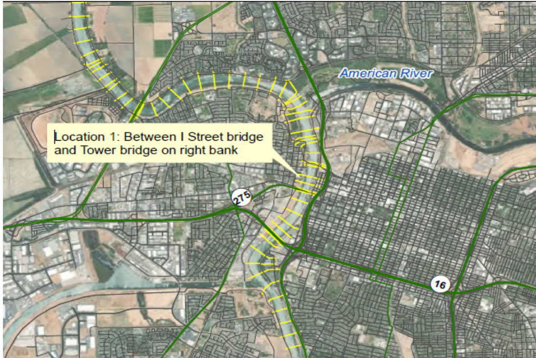
Figure 4-6: High-Water Mark Location 1 – Right Bank Between I Street and Tower Bridges
