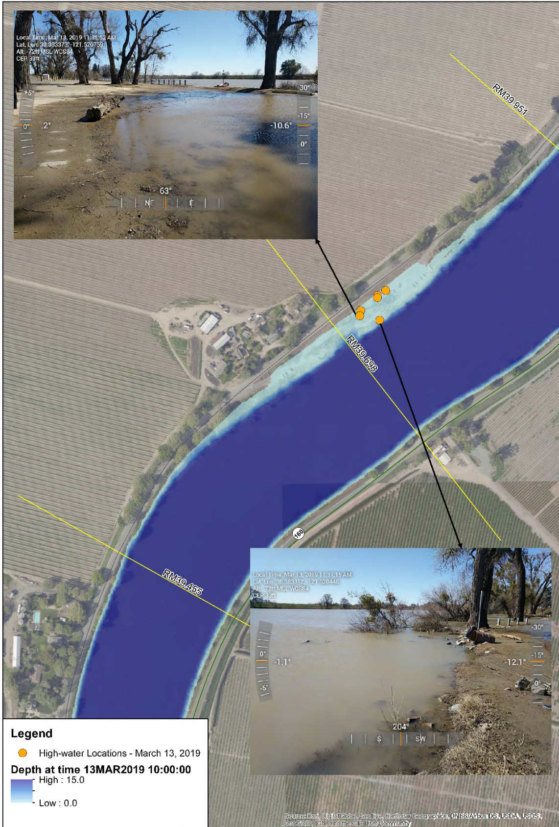
Figure 4-13: High-water Marks at Location 3 - Clarksburg, Mar 13, 2019 at 10:00
