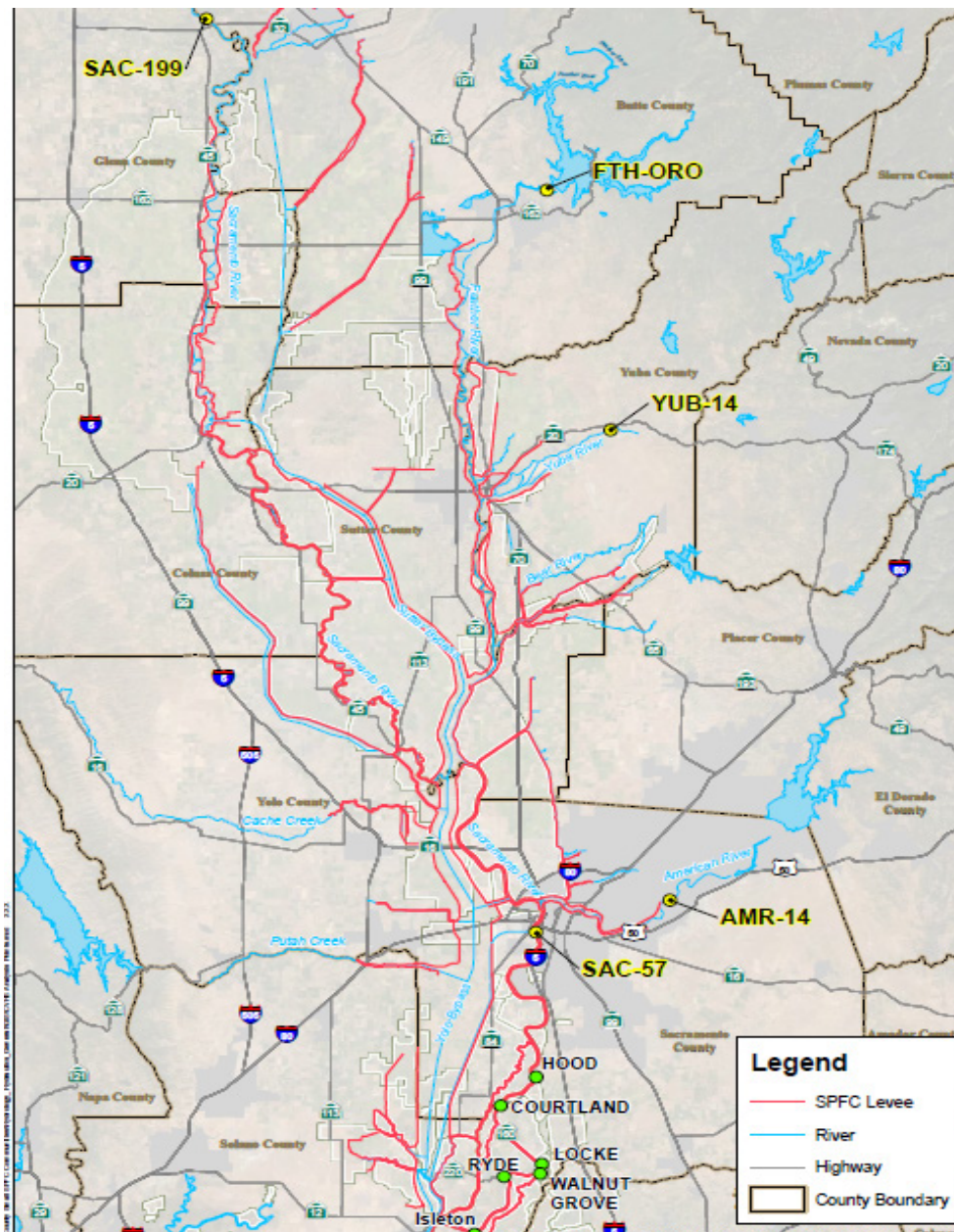
Figure 2-3: CVHS Analysis Points of DWR CVFED Hydraulic Model
